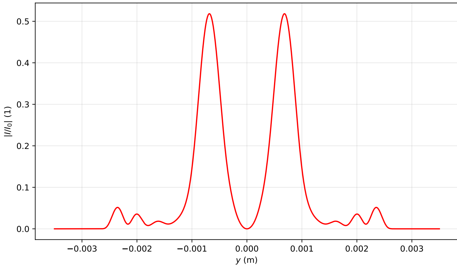
Intensity profile I(x=0, y, z=2.786)/I_0 , P_{in}=6.0P_{cr} , artificial time
